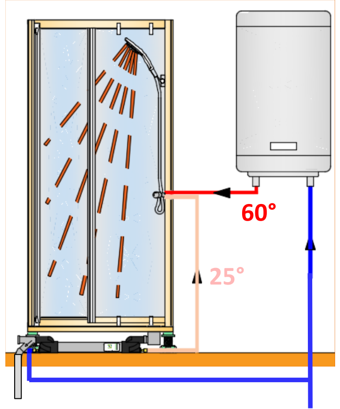
Installation TurboSiphon
